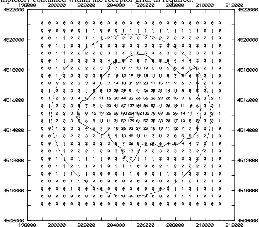
Figure 6. Plot of pollutant concentrations showing the 5 \mu\text{g}/\text{m}^3 significance level and the radius of impact (dashed line circle), determined from the greatest lineal extent of the significance level from the source.
