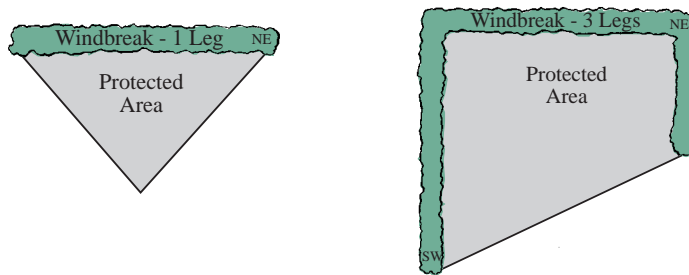
Figure 3. In areas with winds from many directions, multiple-leg windbreaks or windbreak systems provide greater protection to the field or farmstead than single-leg windbreaks.
