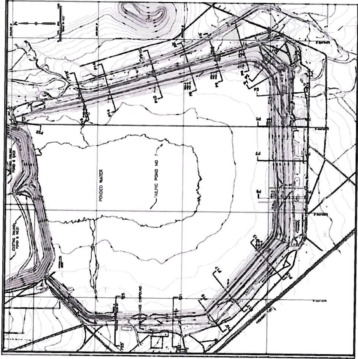
Figure 10. Tailing Pond No. 7 Study Sections
